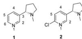
Figure 1. ( S )-Nicotine ( 1 ) and ( S )-6-chloronicotine ( 2 ).
