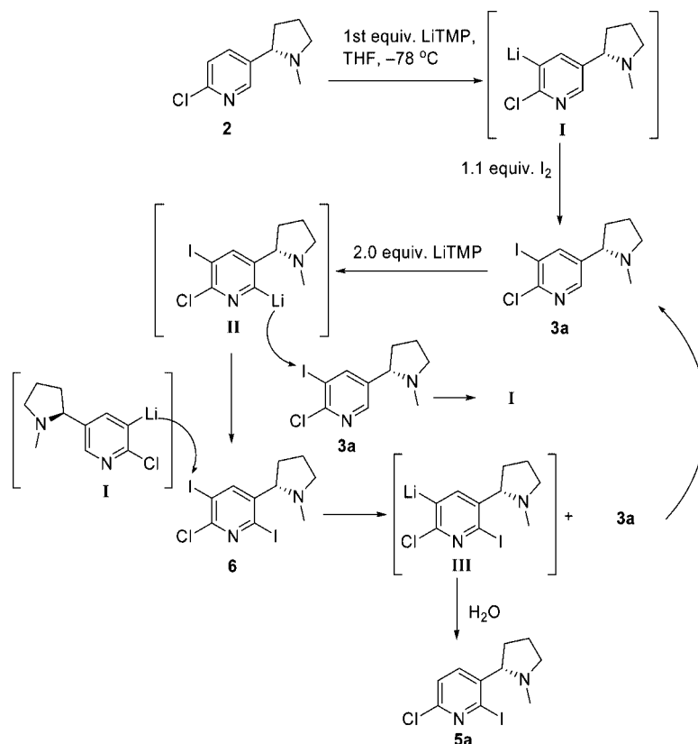
Scheme 1. Proposed mechanism for the formation of 5a by an iodine dance reaction.
