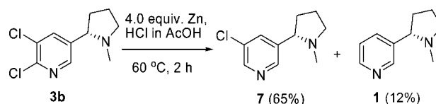
Scheme 2. Regioselective dehalogenation.
